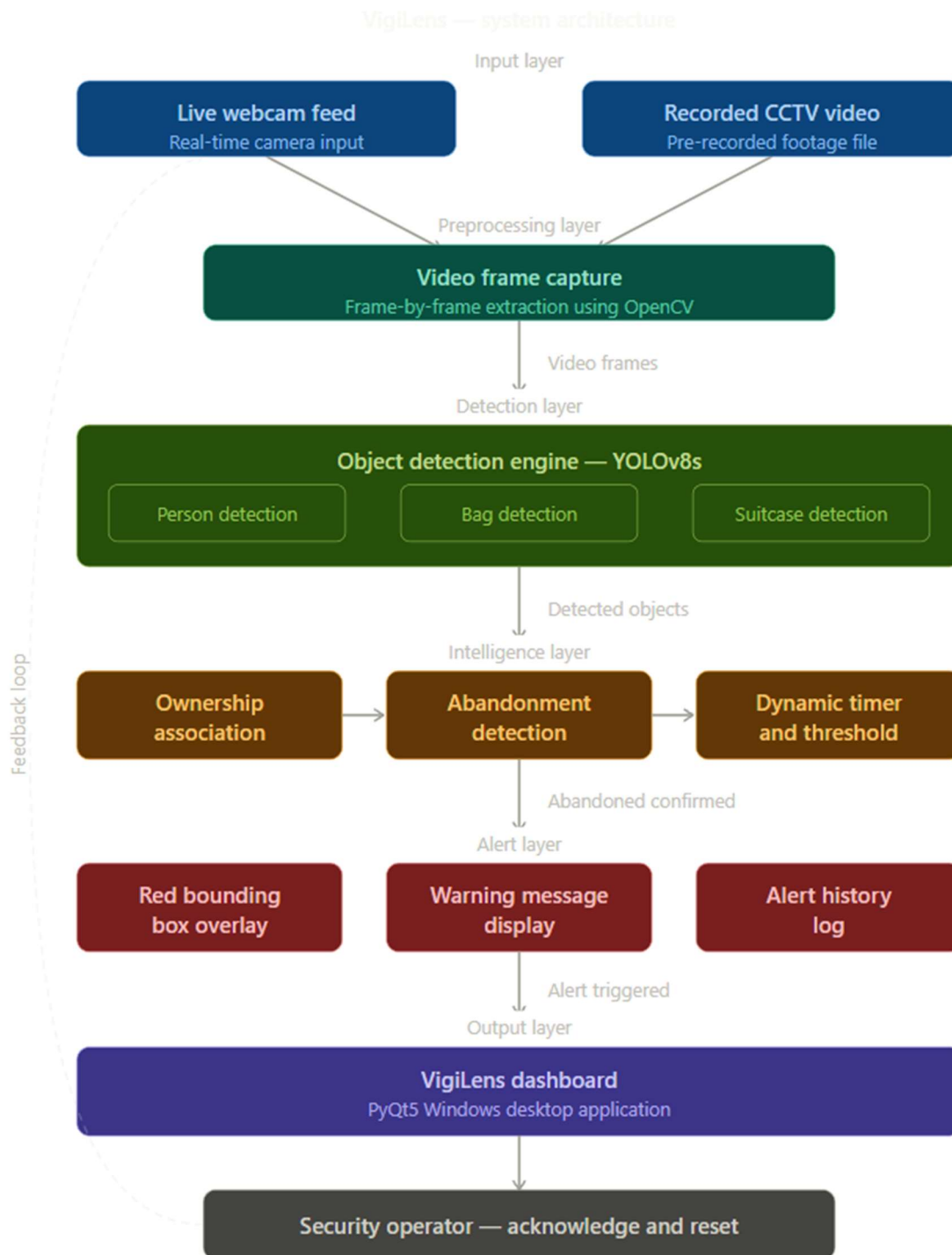
Figure 1: System Architecture Diagram of Vigilens — Real-Time Video Surveillance System for Detection of Abandoned Objects
